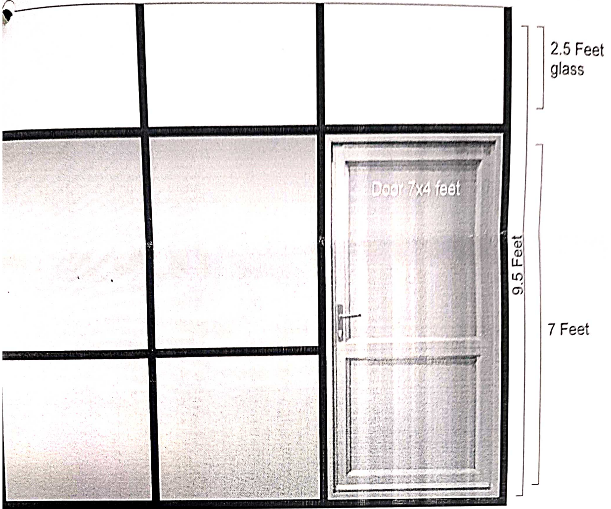
Door Parathion Drawing
